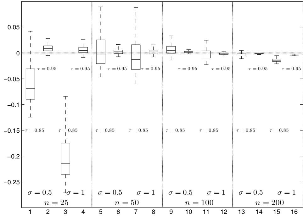
Figure 1: Numerical Example I in Section 3.2. Boxplots of 500 differences \hat{df}_{(s)} - df_{(s)} with s = 2^{p-1} .
