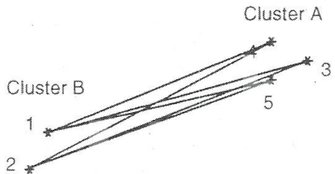
Figure 6.4 Intercluster distance measures.
