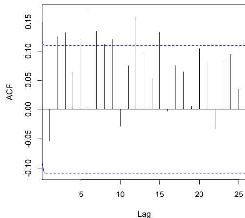
Sample ACF of Residuals from AR(1) Model for Robot Data
