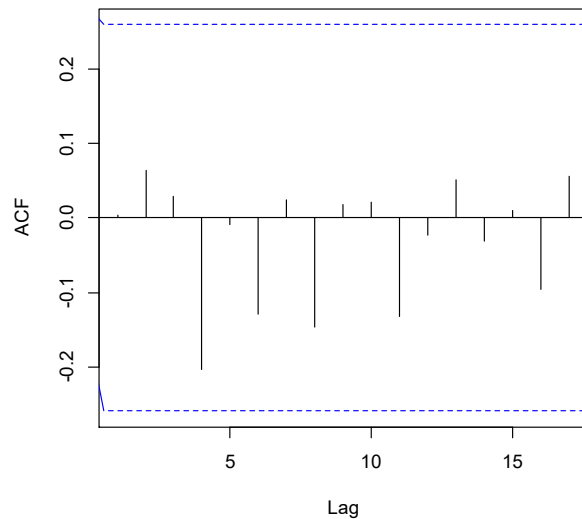
Sample ACF of Residuals from AR(1) Model for Deere Data
