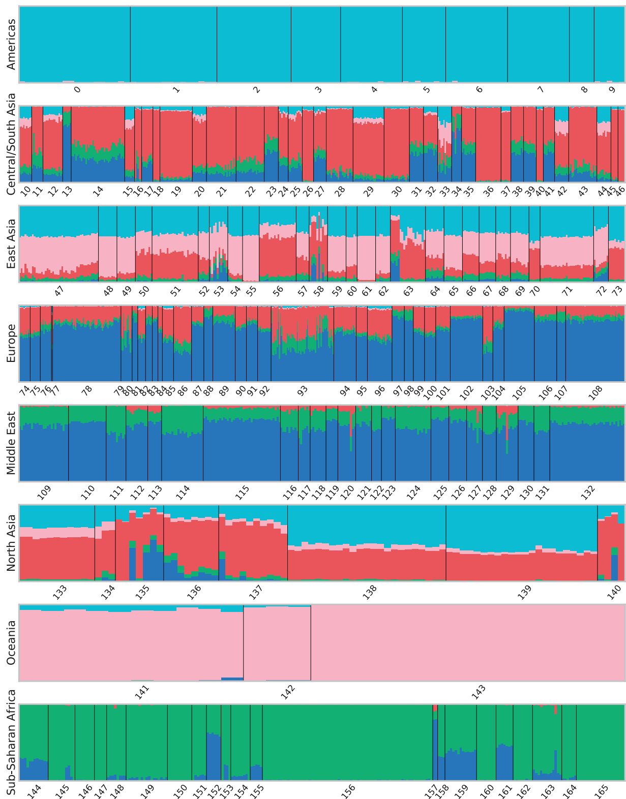
Fig. 6. Genetic clustering results with k=5 clusters using GCAE. Each bar represents a sample from the Human Origins data set, with colors indicating the proportional assignment into k clusters for that sample. Samples are ordered by population and superpopulation, with numbering according to the legend in Fig. 1.
