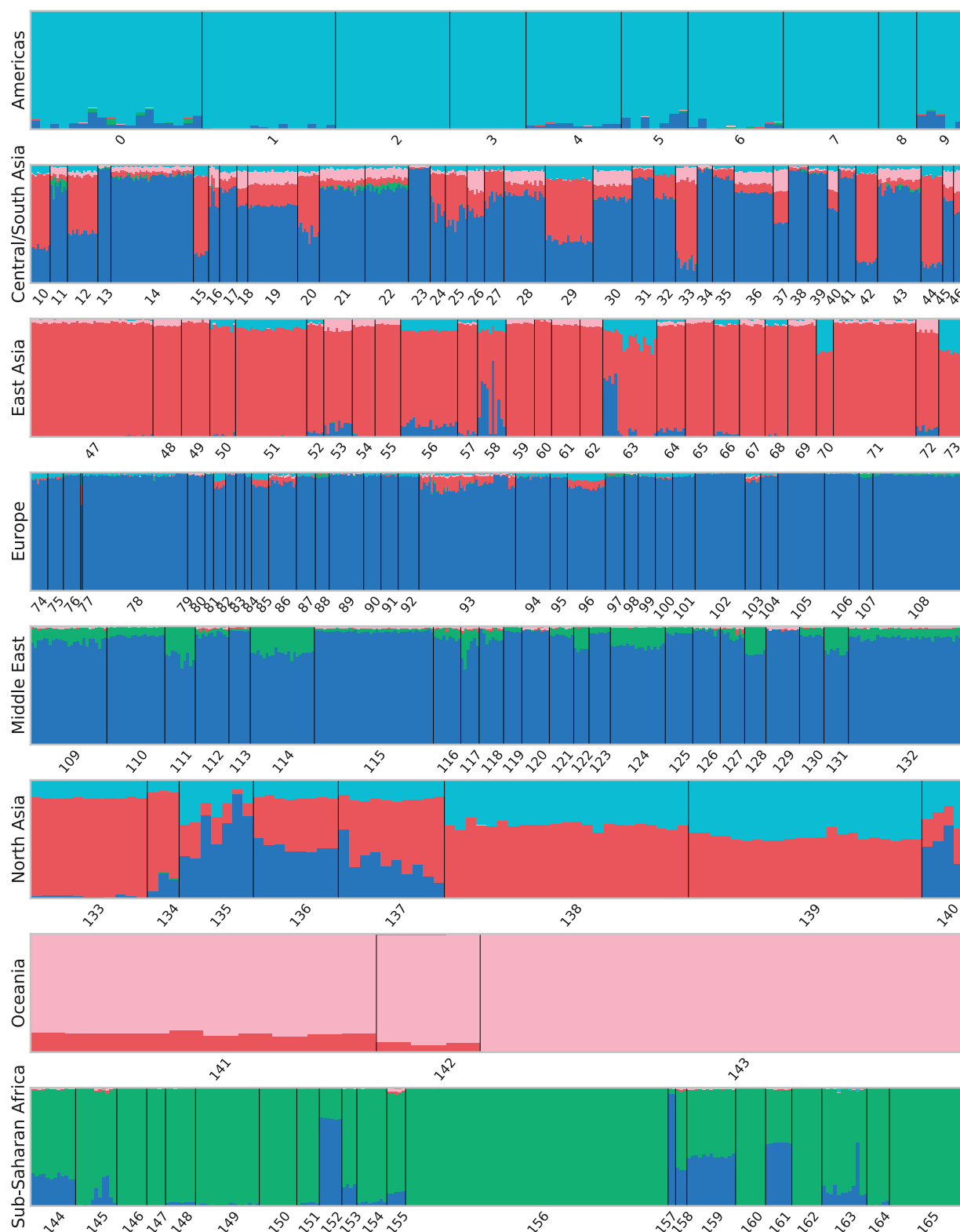
Fig. 5. Genetic clustering results with k = 5 clusters using ADMIXTURE. Each bar represents a sample from the Human Origins data set, with colors indicating the proportional assignment into k clusters for that sample. Samples are ordered by population and superpopulation, with numbering according to the legend in Fig. 1.
